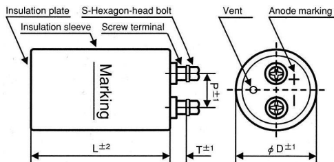
Capacitors with screw terminals series
