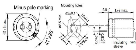
L type(snap in 3 pins):
