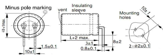
C type(long lead 2 pins):
