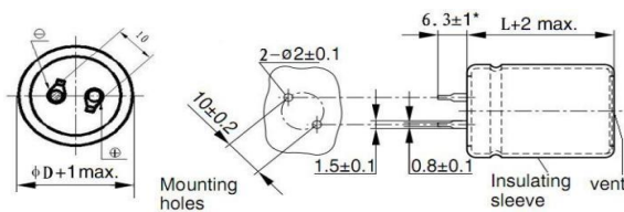
K type(snap in 2 pins):
